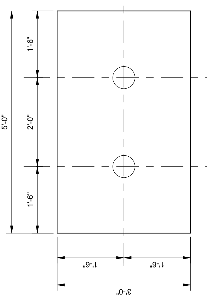
Pile Cap Plan and Section SCALE: 3/4" = 1'-0"
