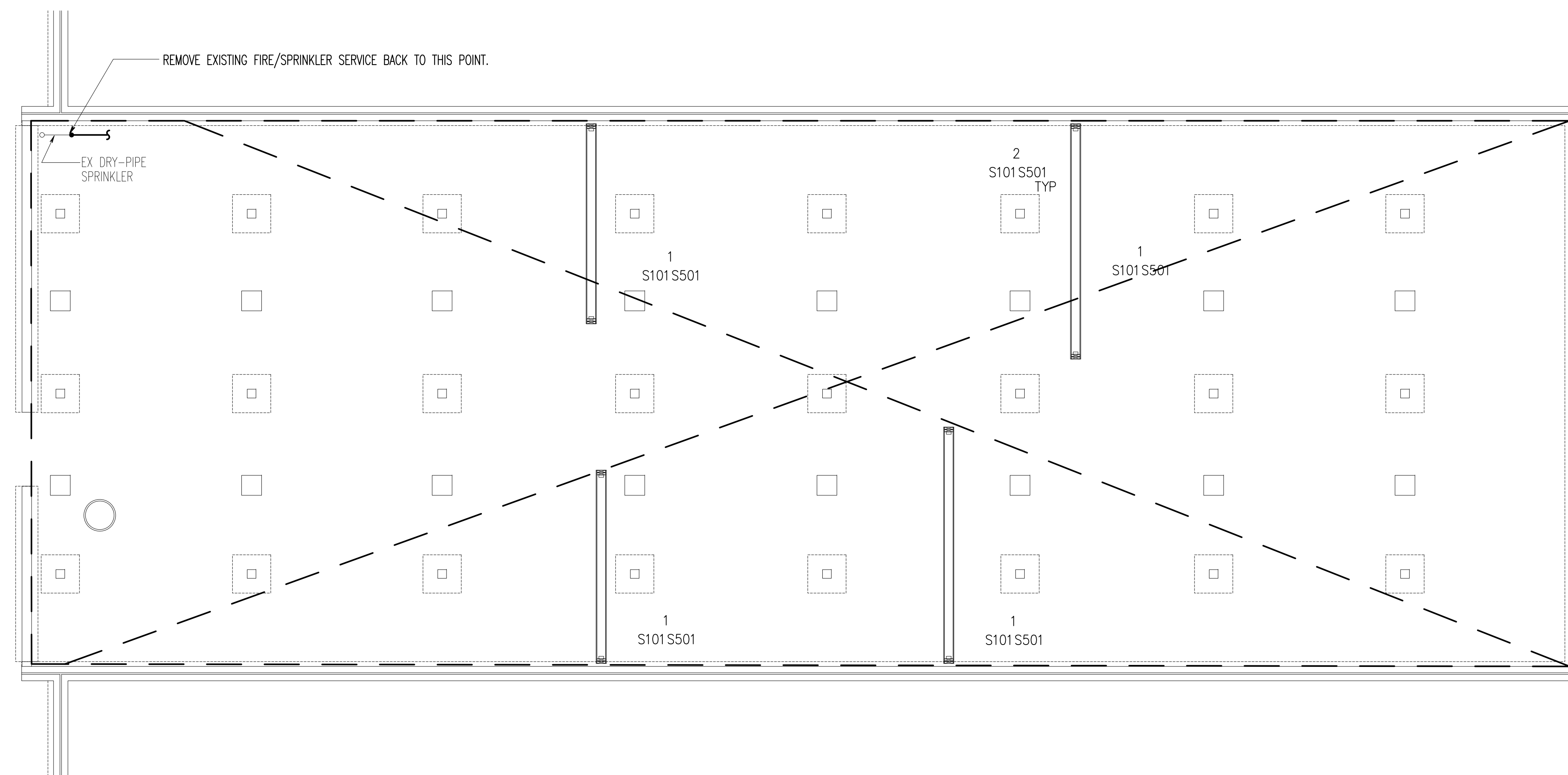
1 CRAWL SPACE PLAN - FIRE PROTECTION DEMOLITION SCALE: 1/4" = 1'-0"
