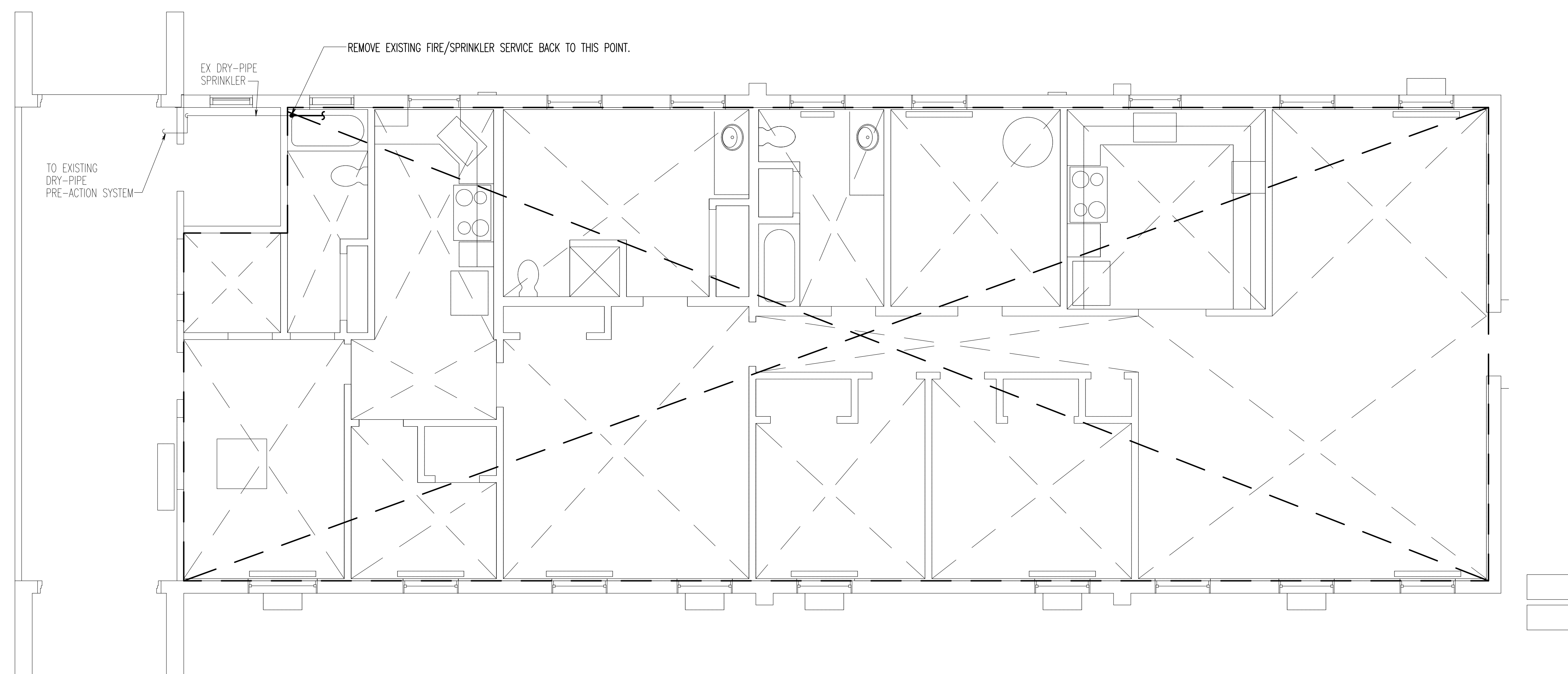
2 FIRST FLOOR & ATTIC PLAN - FIRE PROTECTION DEMOLITION SCALE: 1/4" = 1'-0"
